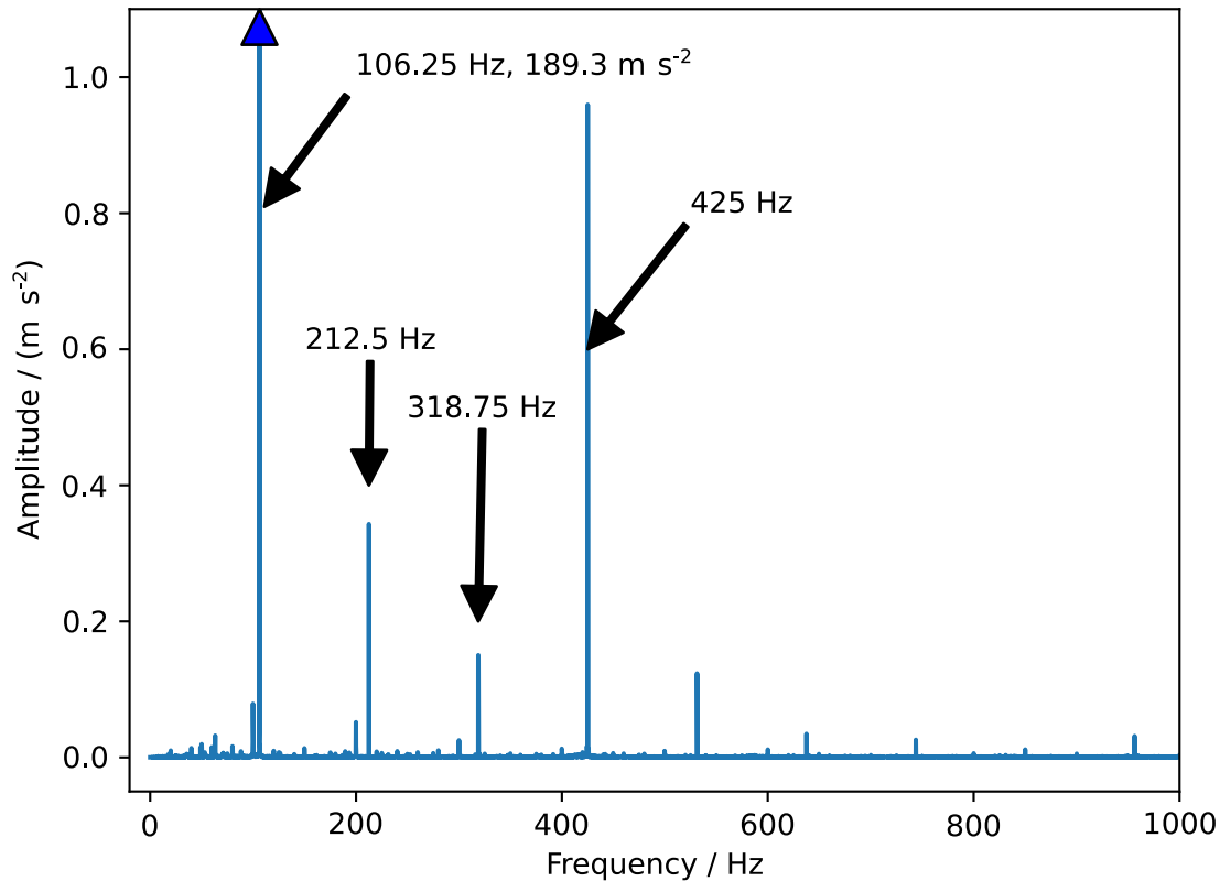
FFT of vibrometer signal
